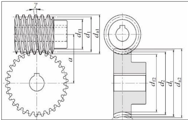
Figure 4: Cylindrical Worm Gear Pair
