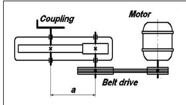
Figure 3: Sketch of Gear Drive
